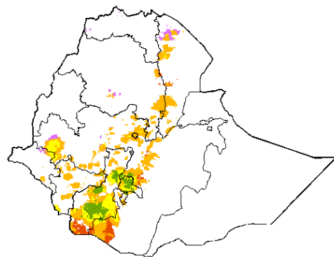
Satellite rainfall estimation
