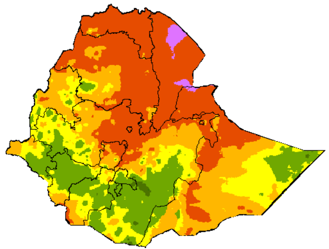
Climatological normal
