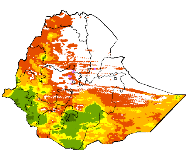
Current dekad
