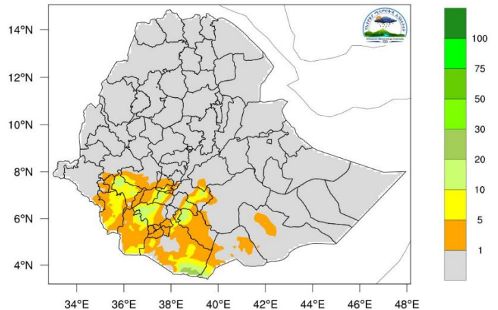
Total Rainfall (mm) for 21 Dec-01 Jan 2025
