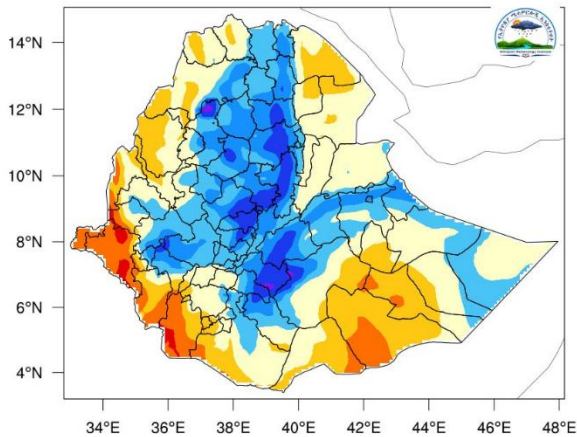
Daily minimum temperature (C) for 21 Dec-01 Jan 2025
