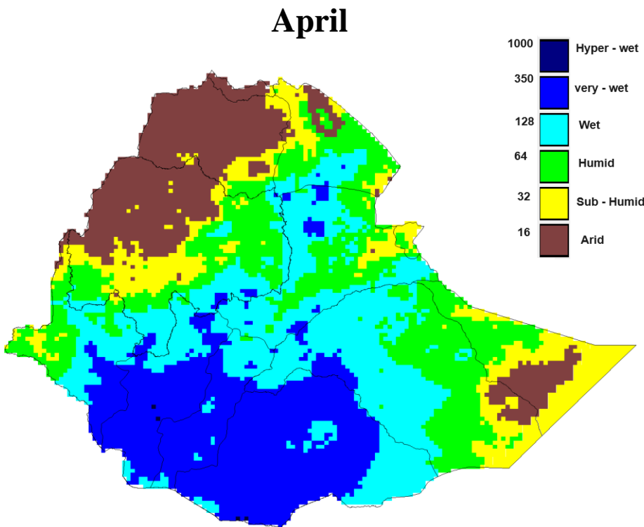
(Fig.3) Aridity Index of April, 2024.
