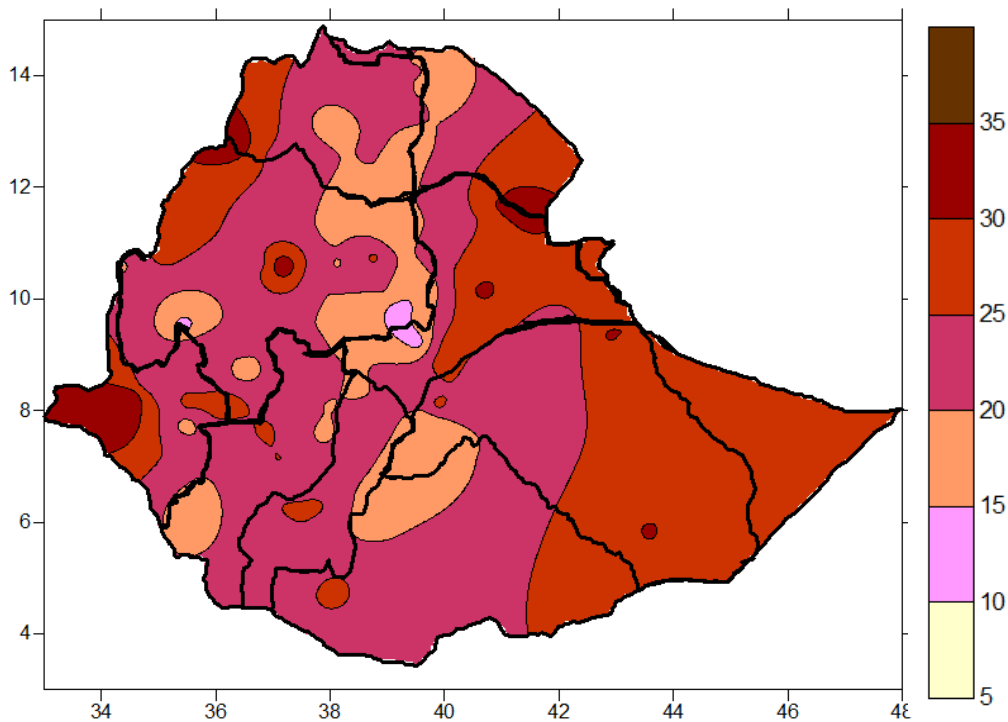
(Fig. 2) Mean monthly Temperature of April, 2024.
