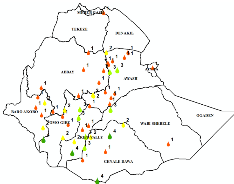
(Fig.4) Distribution and frequency of heavy fall days in April, 2024
