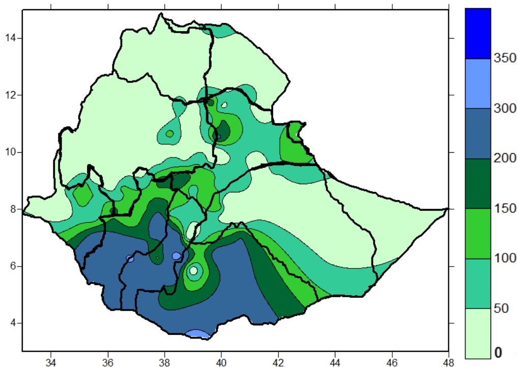
(Fig.1) Monthly precipitation of April, 2024
