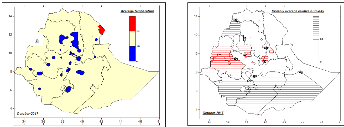
Fig. 2:- Temperature and relative humidity assessment of October 2017
