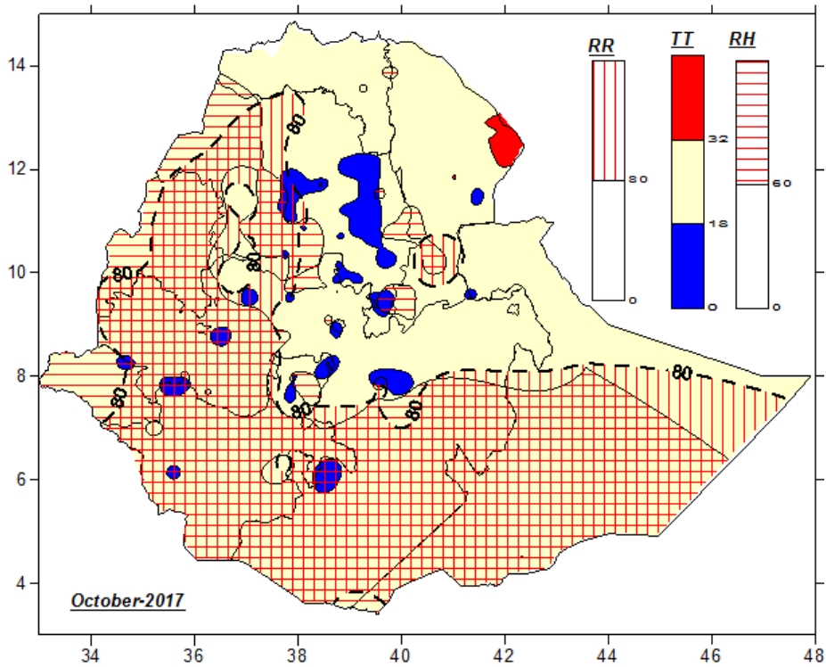
Fig 4:- Combined temperature, rainfall and relative humidity analysis for October 2017. Areas under square patterns with yellowish background color are assumed to satisfy favorable climatic conditions for malaria.
